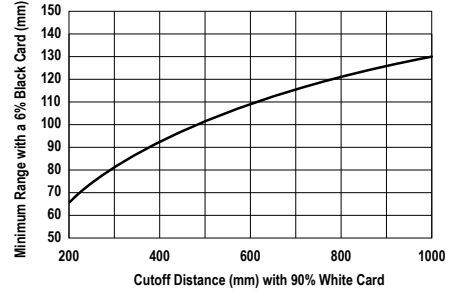
Figure 10. Q60 Minimum Range Versus Cutoff Setting
